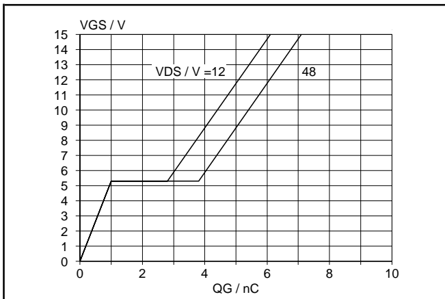
Fig. 13. Typical turn-on gate-charge characteristics. V_{GS} = f(Q_G) ; conditions: I_D = 1.6 \text{ A} ; parameter V_{DS}
