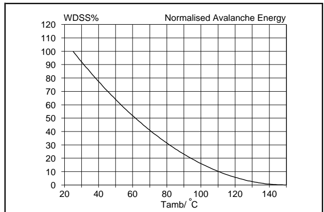
Fig. 15. Normalised avalanche energy rating. W_{DSS}\% = f(T_{amb}) ; conditions: I_D = 1.6 \text{ A}
